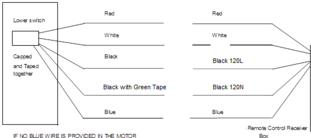
Switch Control box
